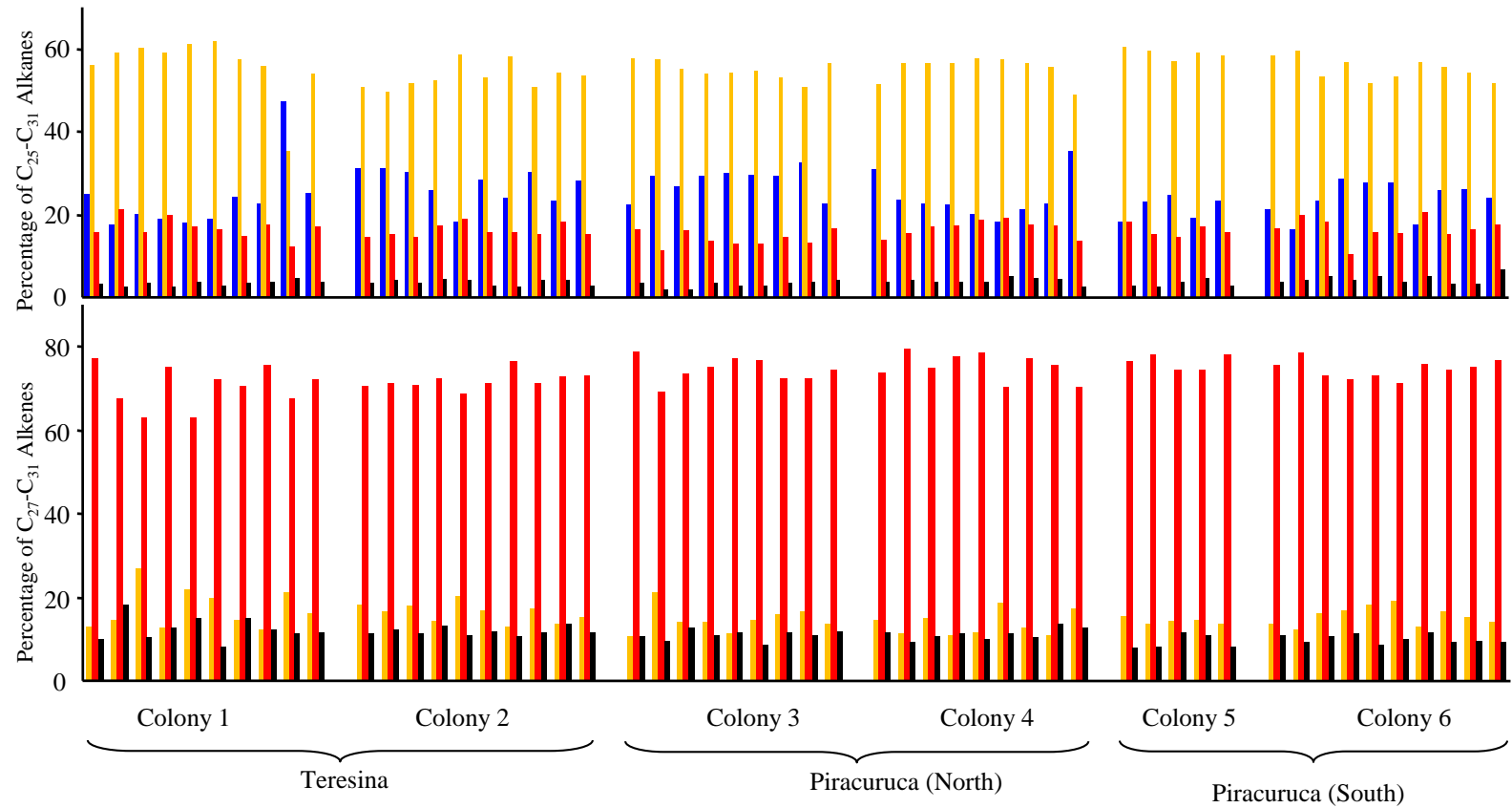
S1. Proportion of alkanes (upper) and alkenes (lower) of 53 individual Melipona fasciculata from six colonies located in 3 meliponaires. Each carbon chain length has a different colour with C 25 =blue, C 27 = yellow, C 29 = red and C 31 = black.
