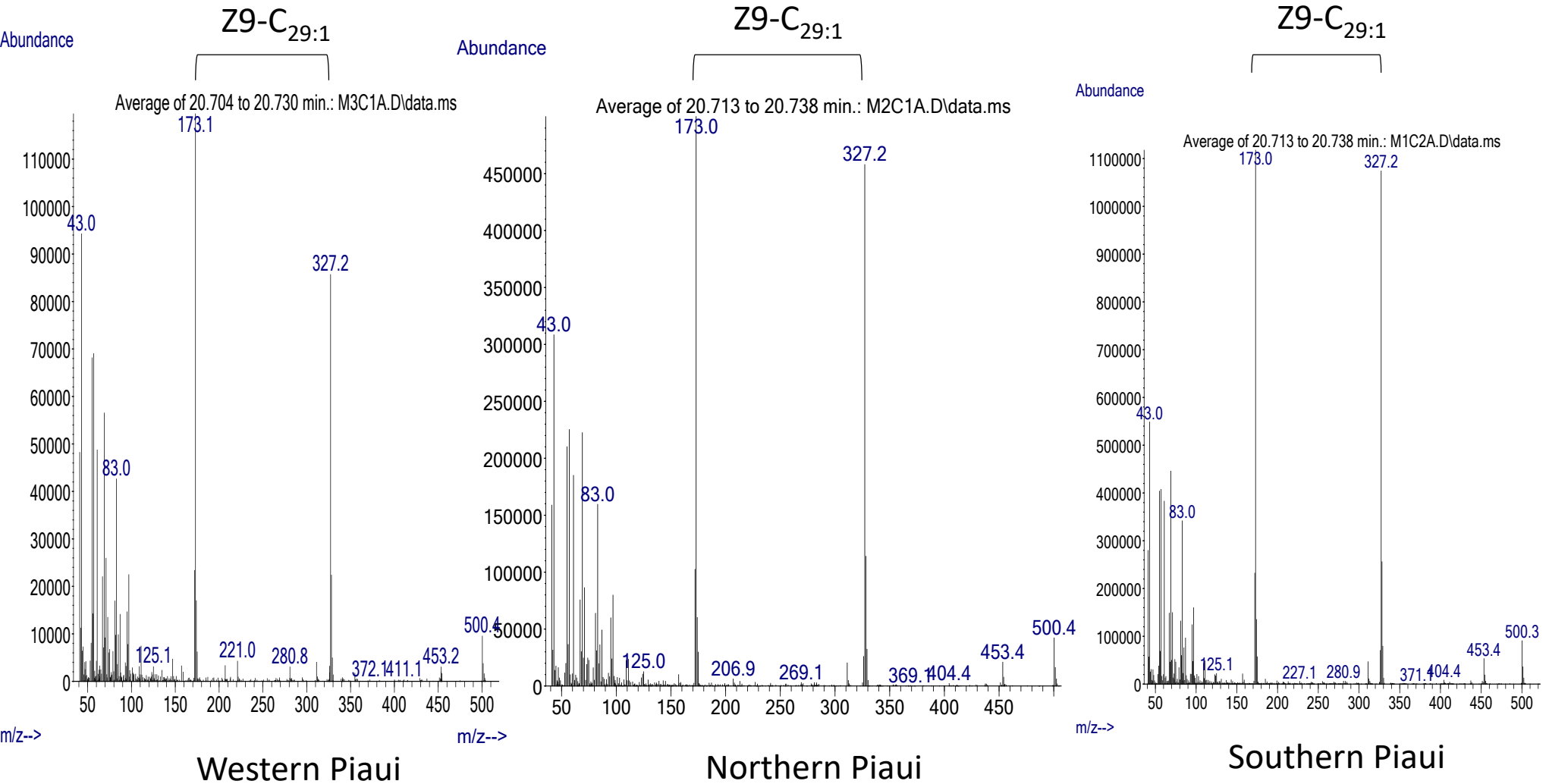
Fig. S2. The fragmentation patterns after a DMDS reaction showing the paired ions associated with the Z9 alkene isomer in M. fasciculata from three different locations across the Brazilian State of Piaui.
