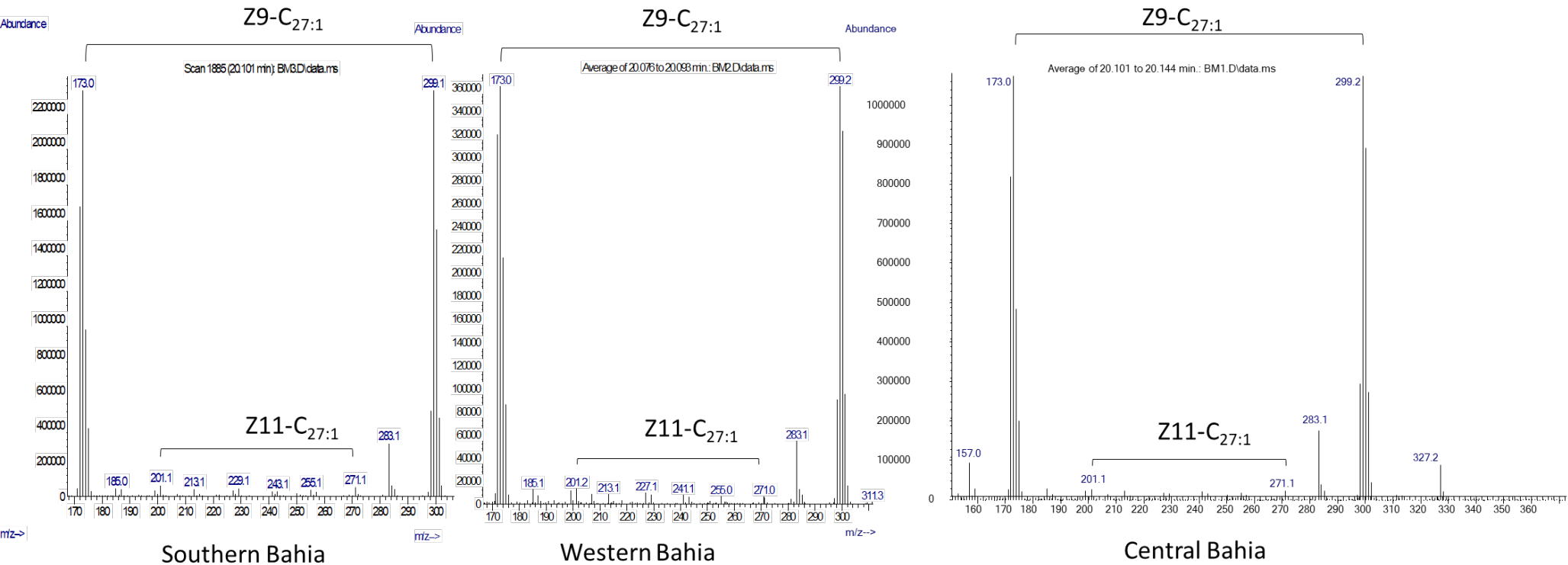
Fig. S3. The fragmentation patterns after a DMDS reaction showing the paired ions associated with the Z11 & Z9 alkene isomers in M. scutellaris from three different locations across the Brazilian state of Bahia.
