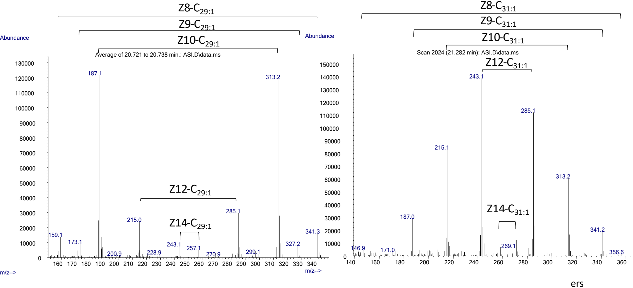
Fig. S6. The fragmentation patterns after a DMDS reaction showing the paired ions associated with the 5 different alkene isomers at two different chain lengths in M. asilvai collected from central Bahai in Brazil
