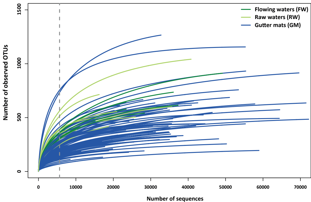
Supplementary Figure 1 | Rarefaction curves for the numbers of observed OTUs defined by at least 99% similarity between 18S rRNA gene sequences for the 104 analyzed samples. To account for differences in sampling efforts, 5,638 sequences (vertical dotted line) were randomly subsampled from each sample.
