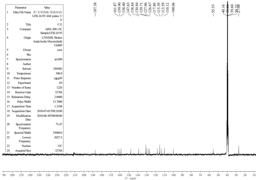
Supplementary Figure 2: 13 C-NMR Spectrum of licochalcone A.
