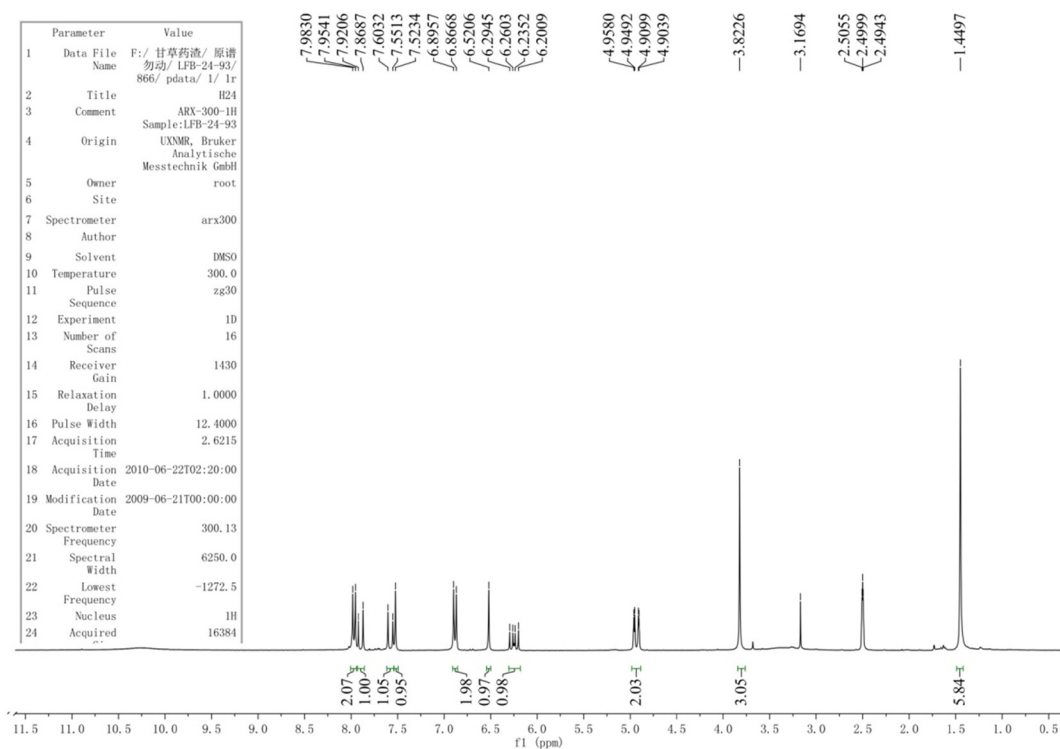
Supplementary Figure 1: 1 H-NMR Spectrum of licochalcone A.
