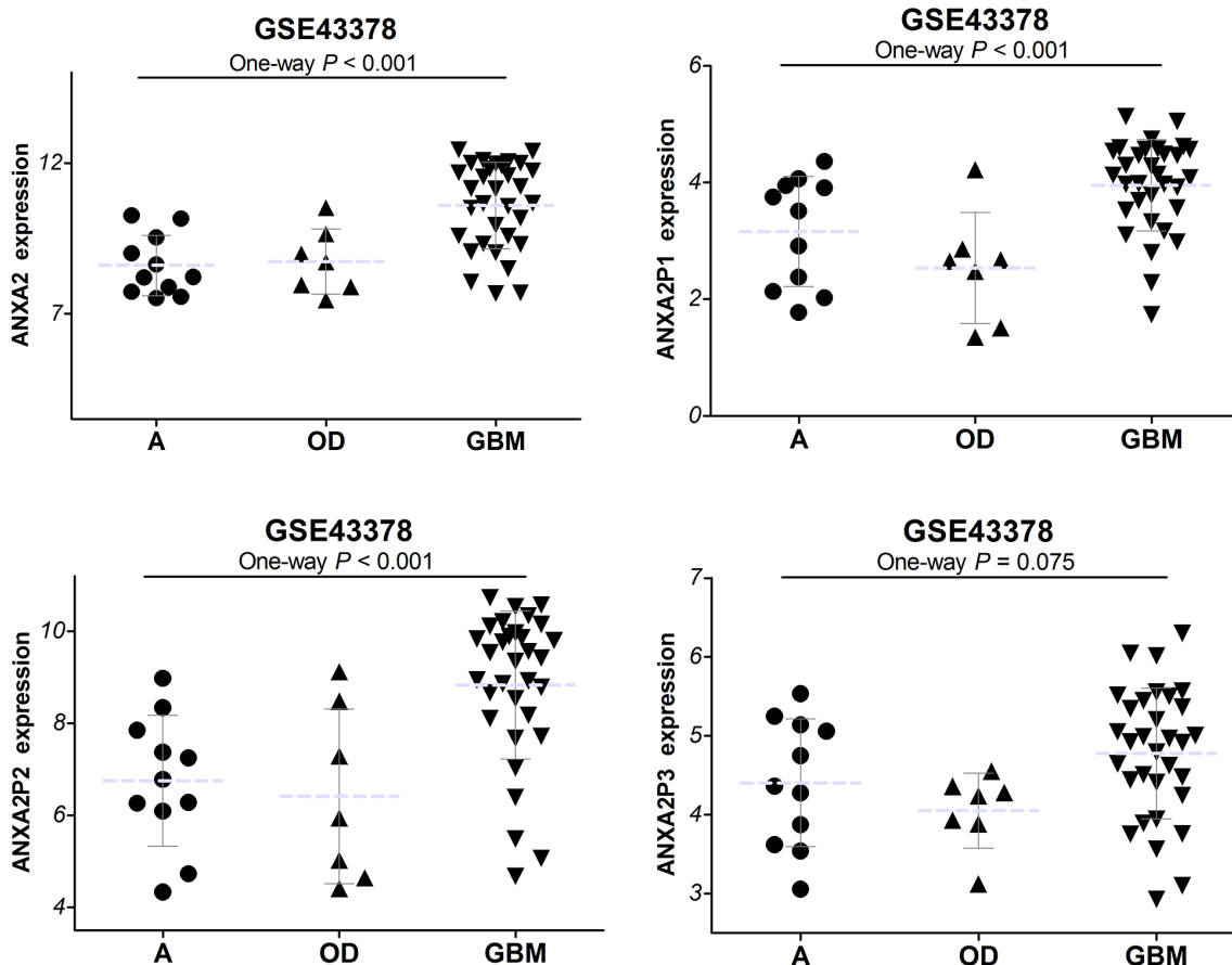
Supplementary Figure 1: ANXA2 and annexin A2 pseudogenes expression in glioma samples of the GSE43378 dataset. Total 50 cases of glioma samples (11 cases of A, 7 cases of OD, 32 cases of GBM).
