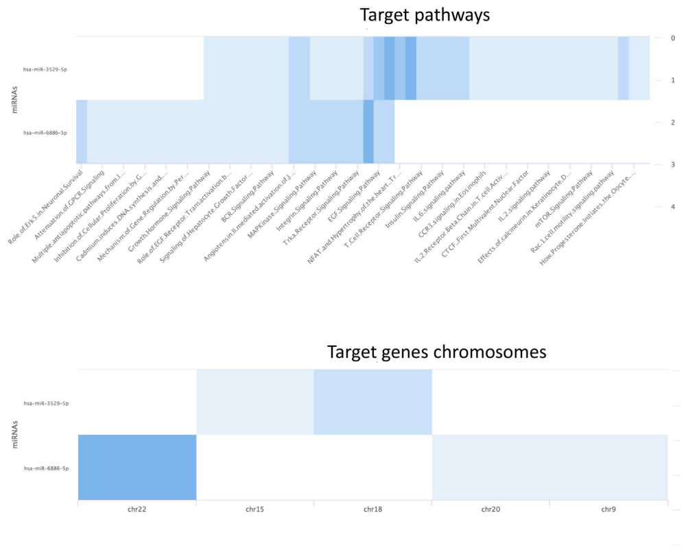
Supplementary Figure 2: Heat map for two miRNAs and target pathways (upper part) and chromosomes (lower part).
