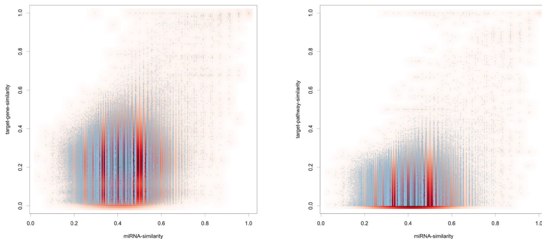
Supplementary Figure 1: Scatter Plot for the miRNA similarity versus target gene similarity (left) and miRNA similarity versus target pathway similarity (right).
