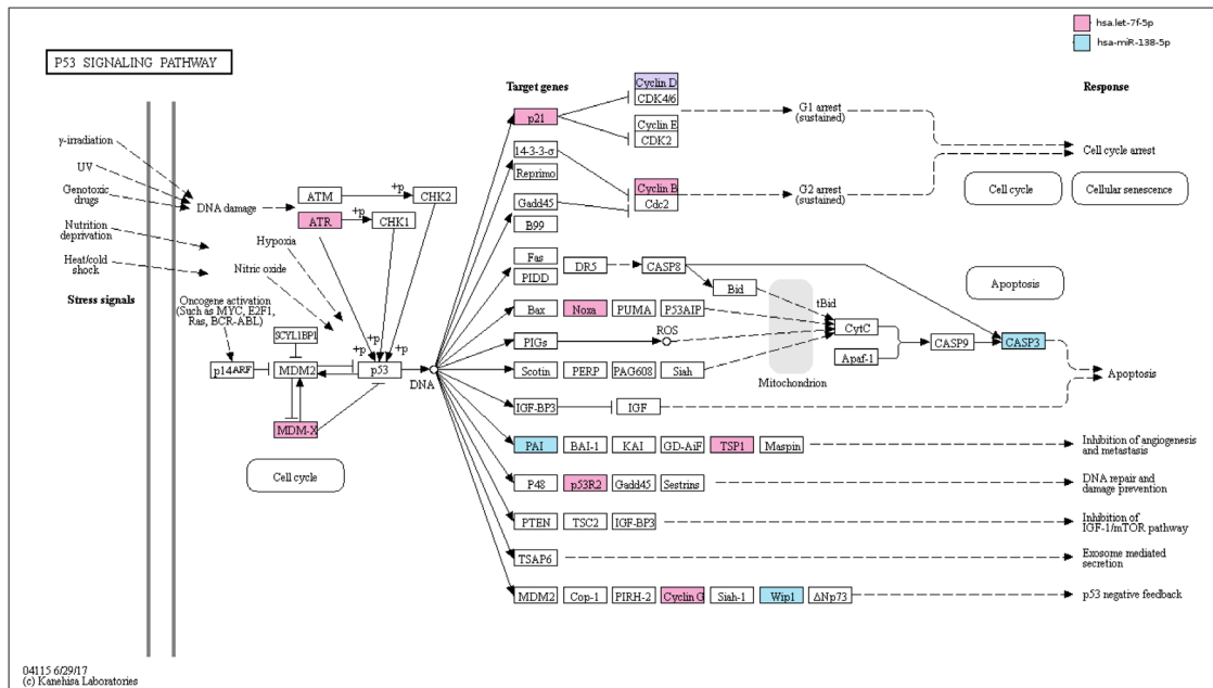
Supplementary Figure 4: experimental targets of the two miRNAs on the p53 signalling cascade. Targets are highlighted in different colors, only one purple target overlaps between both miRNAs.
