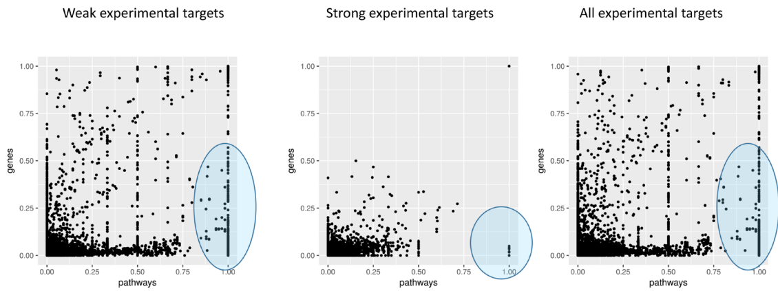
Supplementary Figure 3: Scatter plots of target pathway versus target gene gene similarity for weak evidence targets (left panel), strong evidence targets (middle panel) and all targets with experimental evidence (right panel). The area of interest described in the manuscript is highlighted in blue.
