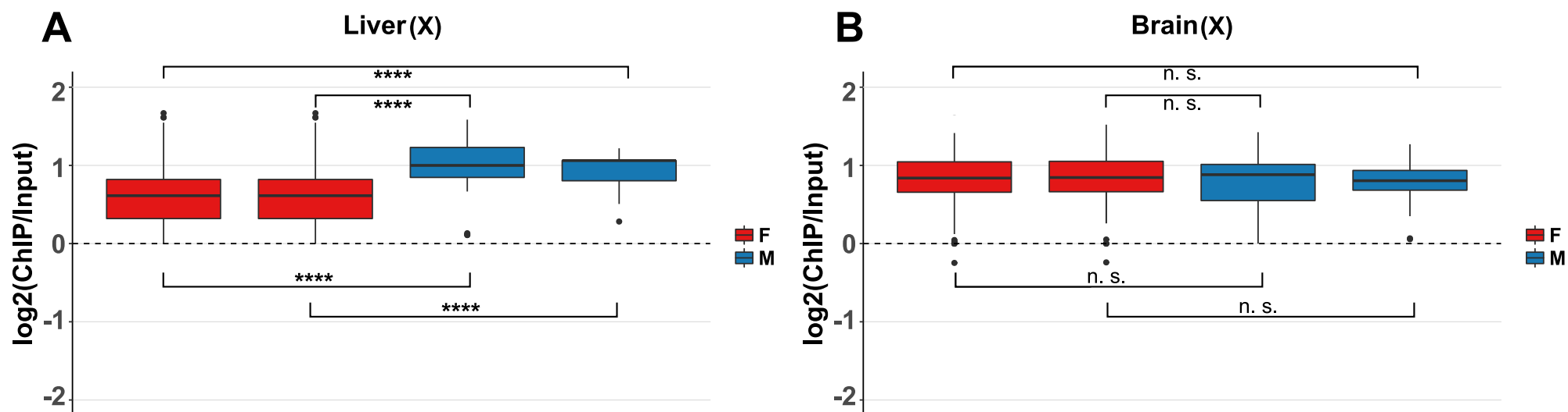
Supplemental Figure S14. Comparisons of H4K16ac enrichment levels on the X chromosome. Comparison of H4K16ac enrichment levels on genic regions of the X chromosome between males (actual levels; see figure 6B) and females (using half of the reads mapping to input) for liver (A) and brain (B). Mann-Whitney U test with FDR correction. ****: P \leq 10^{-5} ; n.s.: P > 0.05 . F=Female M=Male.
