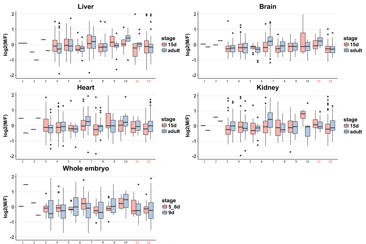
Supplemental Figure S7. Male-to female \log_2 -gene expression ratio for X-linked contigs. Contigs GL343947.1 (11) and LGb (12) do not show higher M:F ratio than other contigs in any of the analyzed tissue/stage, contrary to what was previously proposed (Rupp et al. 2017). Numbers on the X-axis indicate the different contigs, as previously defined (Alfoldi et al. 2011): 1 = AAWZ02038267, 2 = AAWZ02041083, 3 = AAWZ02038845, 4 = GL343282.1, 5 = GL343338.1, 6 = GL343364.1, 7 = GL343417.1, 8 = GL343423.1, 9 = GL343550.1, 10 = GL343913.1, 11 = GL343947.1, 12 = LGb.
