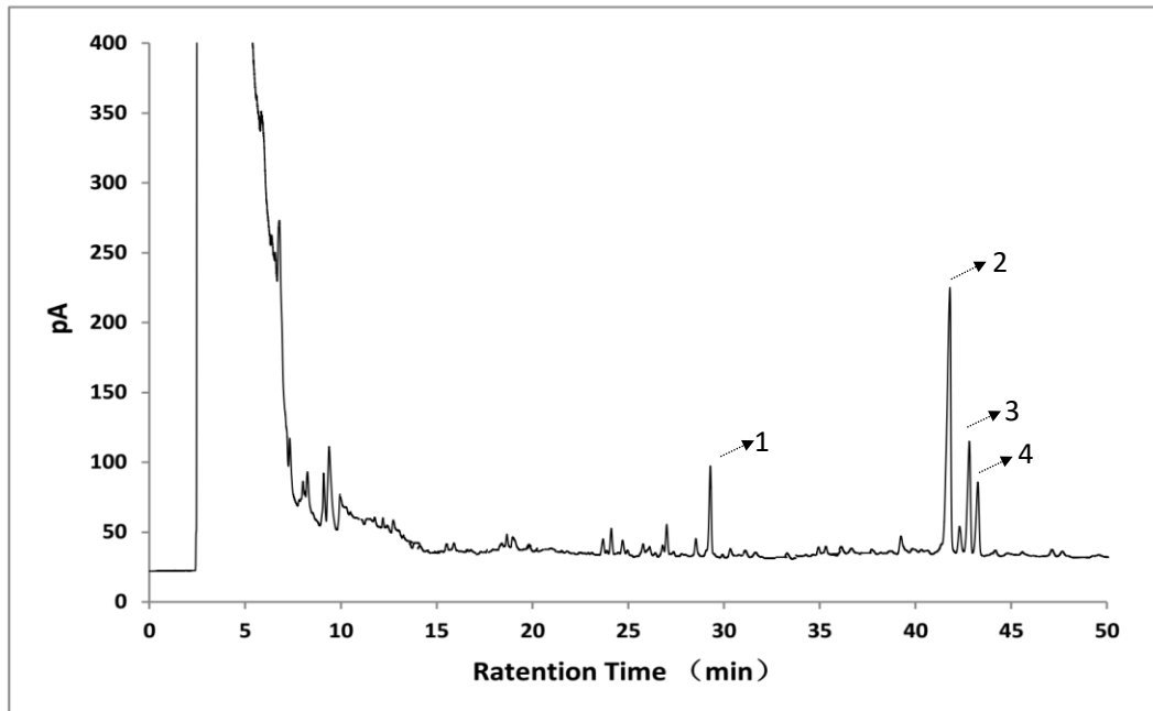
Supplement data 1. GC spectrum of monosaccharide composition of EPCP1-2.
