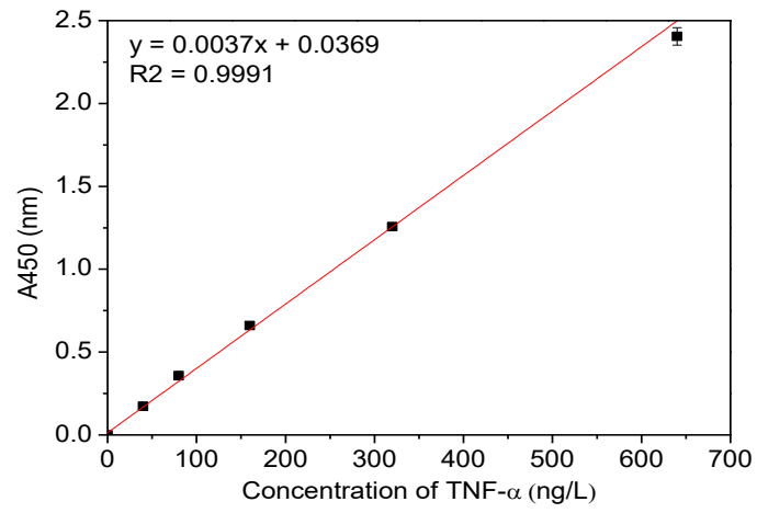
Supplement data 2. Standard curve of cytokines protein expression by Elisa (a) IL-1 \beta (b) IFN- \gamma (c) TNF- \alpha
