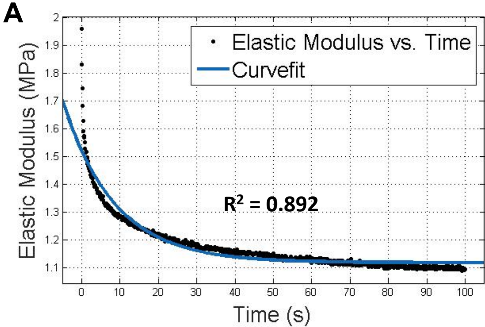
Curve fitting to a Standard solid viscoelastic model
