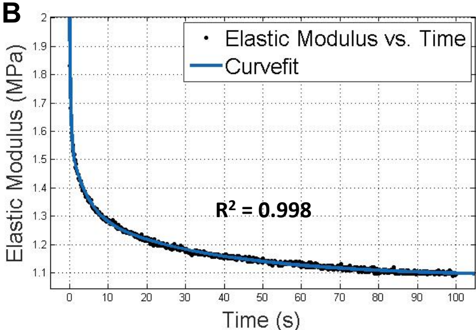
Curve fitting to a Prony series
