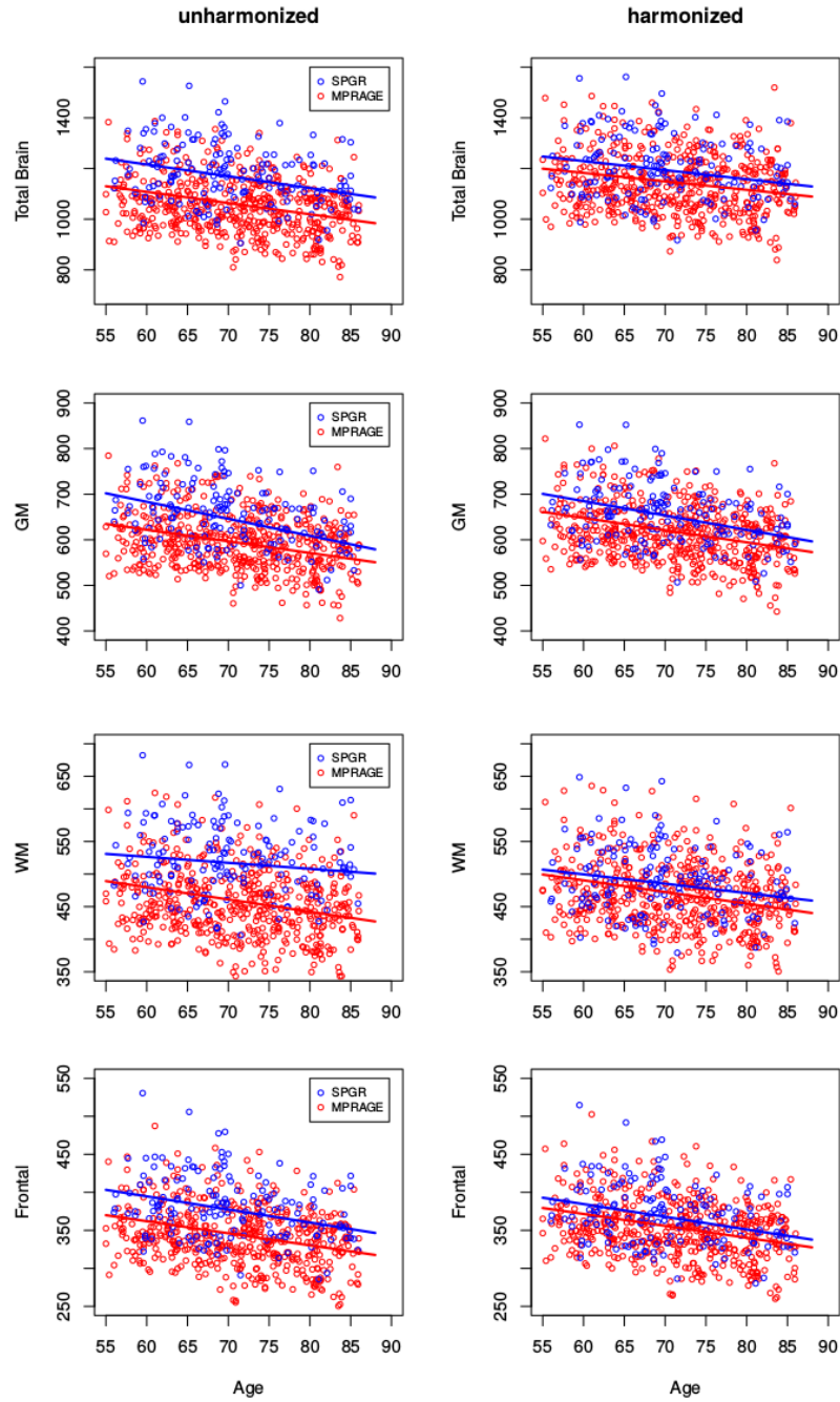
Fig.S. 1: Cross-sectional age trends for total brain, GM, WM and the frontal lobe (GM and WM together) for the two scanner types, and for harmonized and unharmonized values. The values in y axis are in cc.
