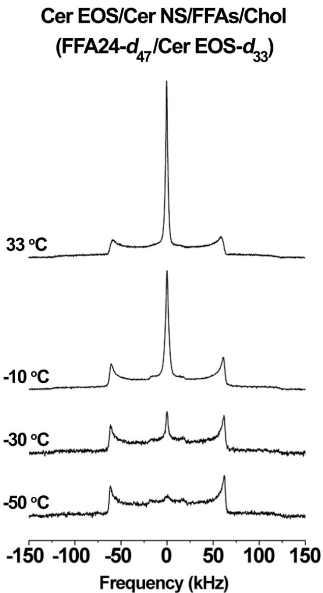
Supplemental Figure S3. ^2\text{H} -NMR spectra of the Cer EOS/Cer NS/FFAs/Chol mixture with both deuterated FFA24- d_{47} and Cer EOS- d_{33} measured at different temperatures.
