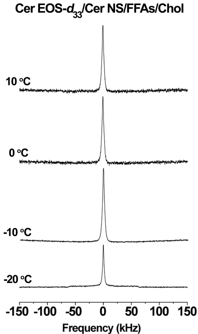
Supplemental Figure S2. ^2\text{H} -NMR spectra of the dehydrated Cer EOS- d_{33} /Cer NS/FFAs/Chol mixture measured at different temperatures.
