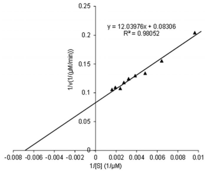
S6 Fig. Evaluation of Michaelis-Menten constant and maximum reaction rate. Total enzyme concentration used for enzyme kinetics was 0.1275 \mu\text{M} .
