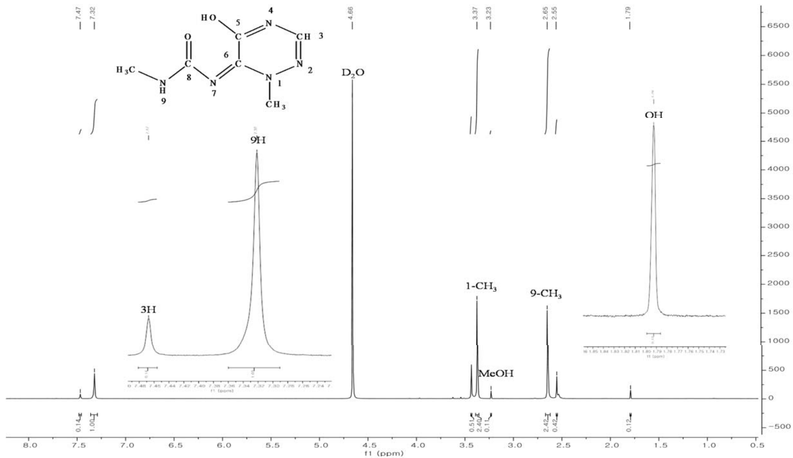
S9 Fig. ^1\text{H-NMR} of degrading products from TXE in \text{D}_2\text{O} . Insert shows peak assignments based on the final structure and enlargement of the spectrum.
