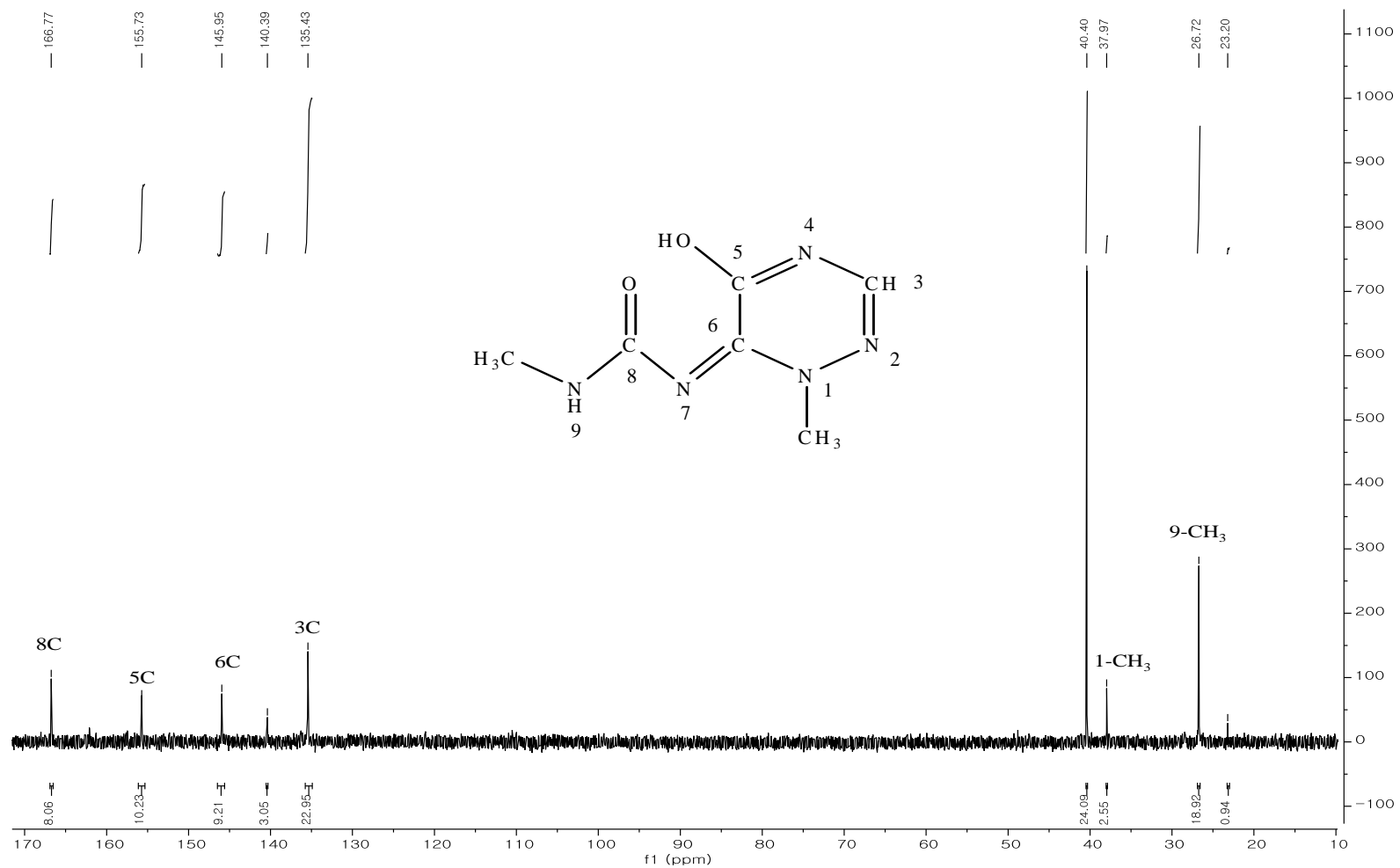
S10 Fig. 13 C-NMR of degrading products from TXE in D 2 O. Insert shows peak assignments based on the final structure and enlargement of this spectrum.
