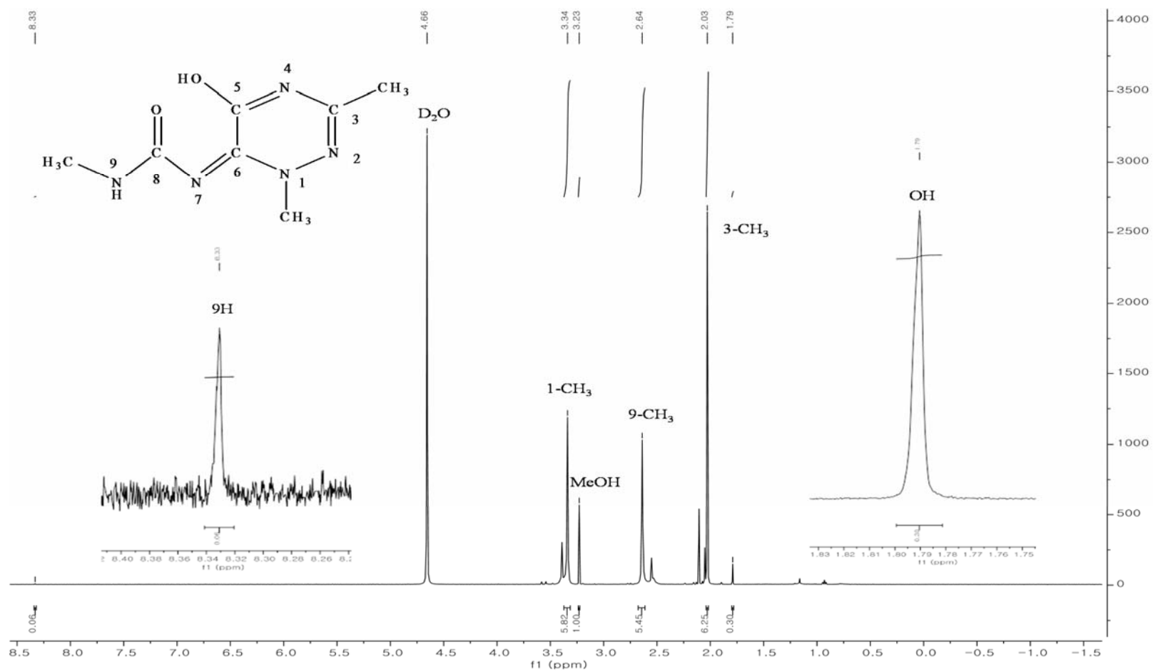
S11 Fig. 1 H-NMR of degrading products of methyltoxoflavin from TXE in D 2 O. Insert shows peak assignments based on the final structure and enlargement of the spectrum.
