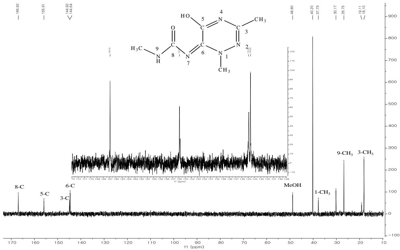
S12 Fig. ^{13}\text{C} -NMR of degrading product of methyltoxoflavin from TXE in \text{D}_2\text{O} . Insert shows peak assignments based on the final structure and enlargement of the spectrum.
