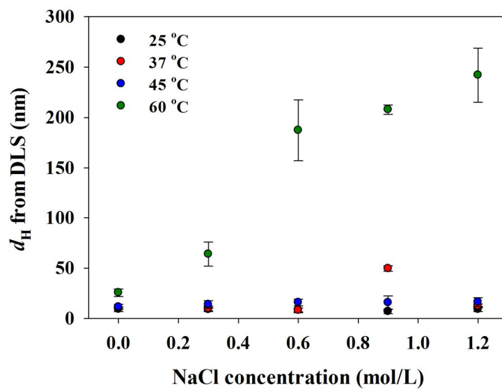
Fig. S1 Variation of d_H with salt concentrations at various temperatures and salt types
