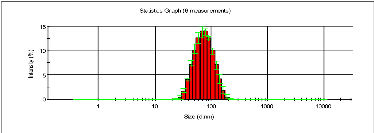
DLS size distribution (intensity) of MCP 1
