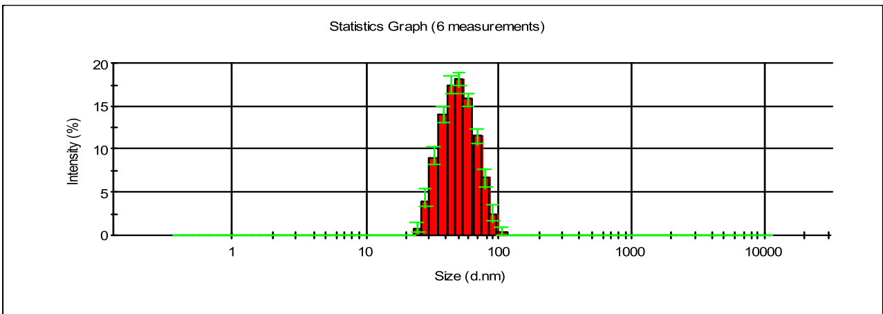
DLS size distribution (intensity) of MCP 2-1
