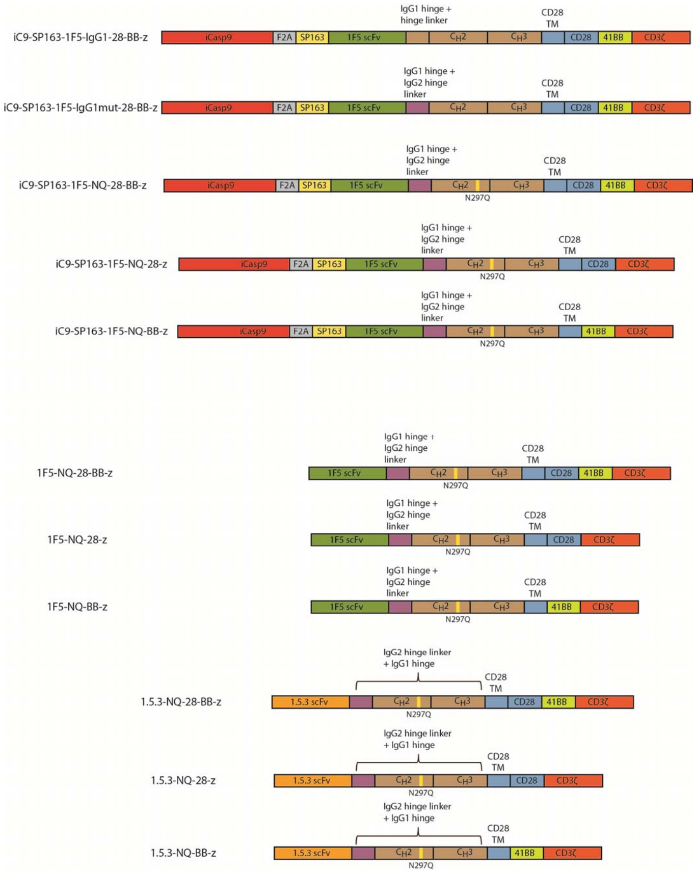
Figure S1. Schematic diagrams of selected CD20 CAR constructs.
