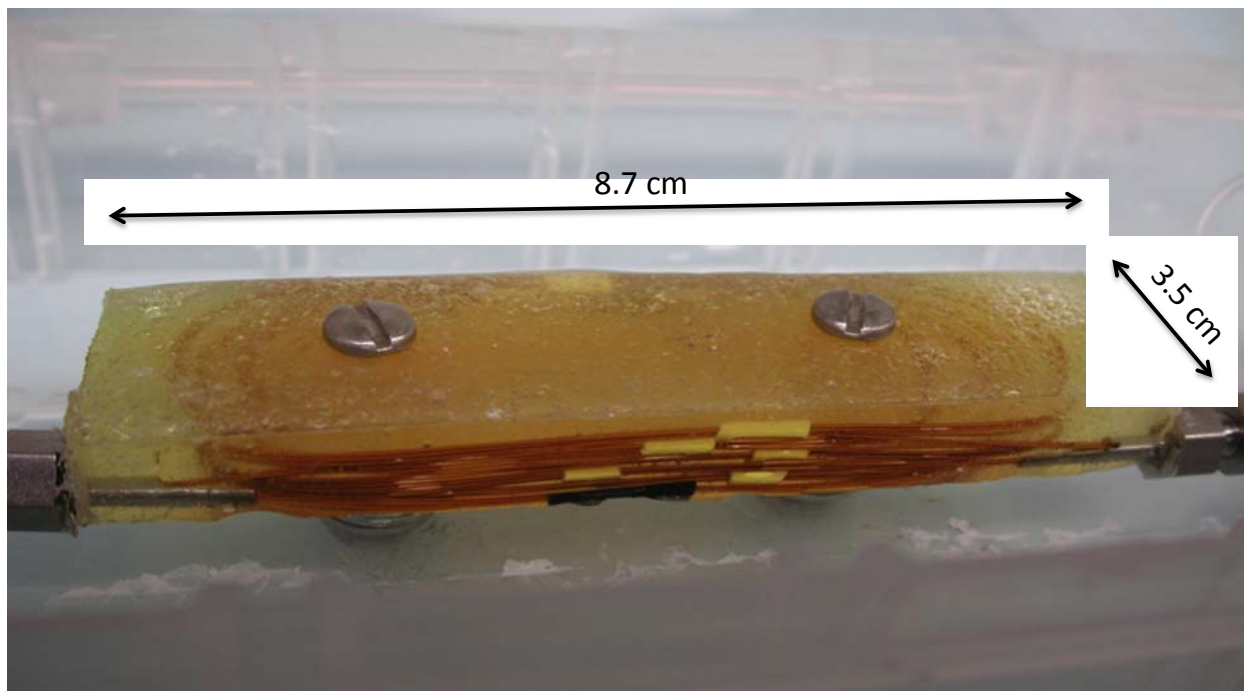
Figure S1: A photograph of a six capillary multi-PLOT-cryo module equipped with compression fittings for use as a headspace vapor collection device.
