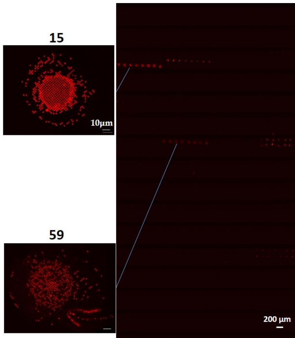
Supplementary Figure 3. Fluorescence micrograph of the liquid lipid based microarray 1hr after immersion under water; which shows the effect of immersion under water on samples stability.
