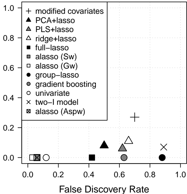
Scenario 6a + correlation 0.6 between the treatment-effect modifiers
