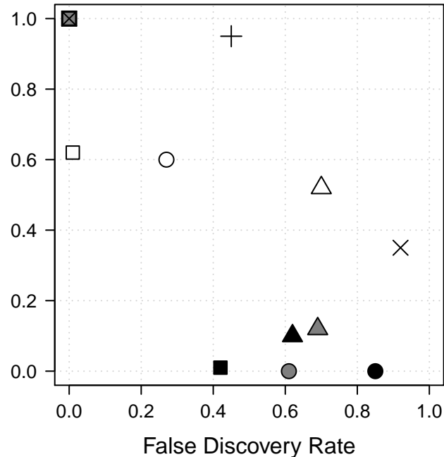
Scenario 6a + correlation 0.6 between all the active markers
