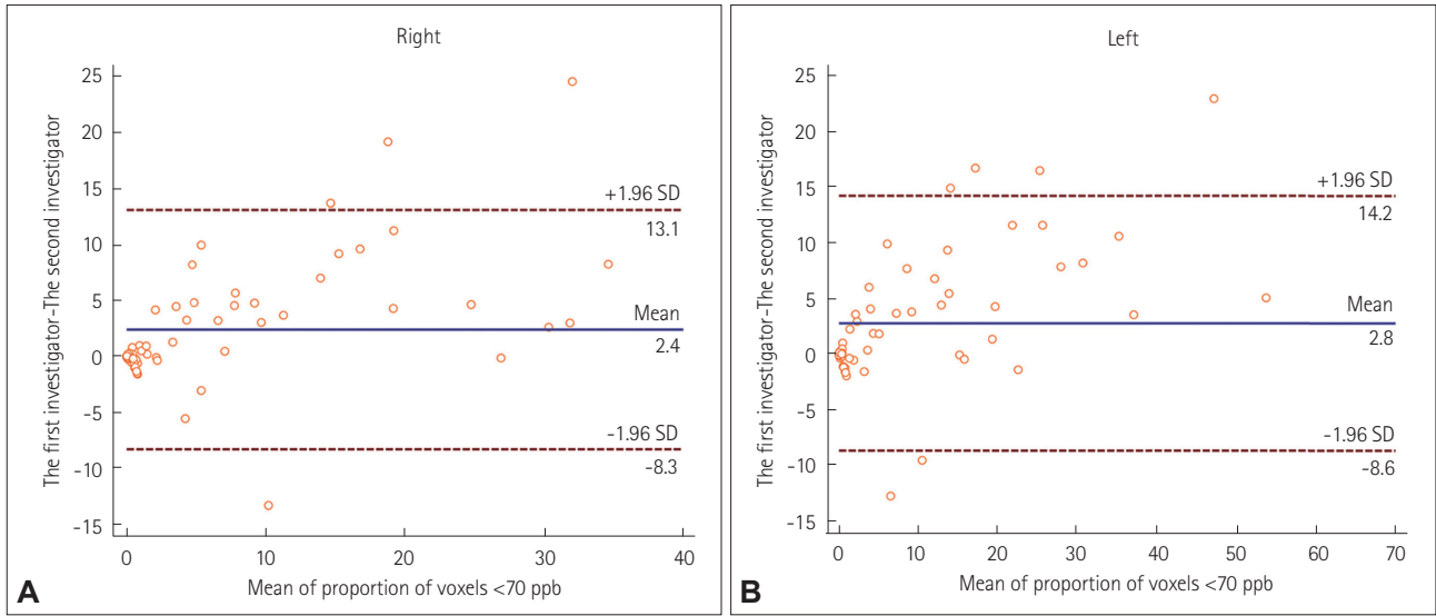
Supplementary Fig. 4. The Bland-Altman plots between the two investigators for the measurement of the proportion of voxels less than 70 ppb in the right (A) and left (B) substantia nigra.
