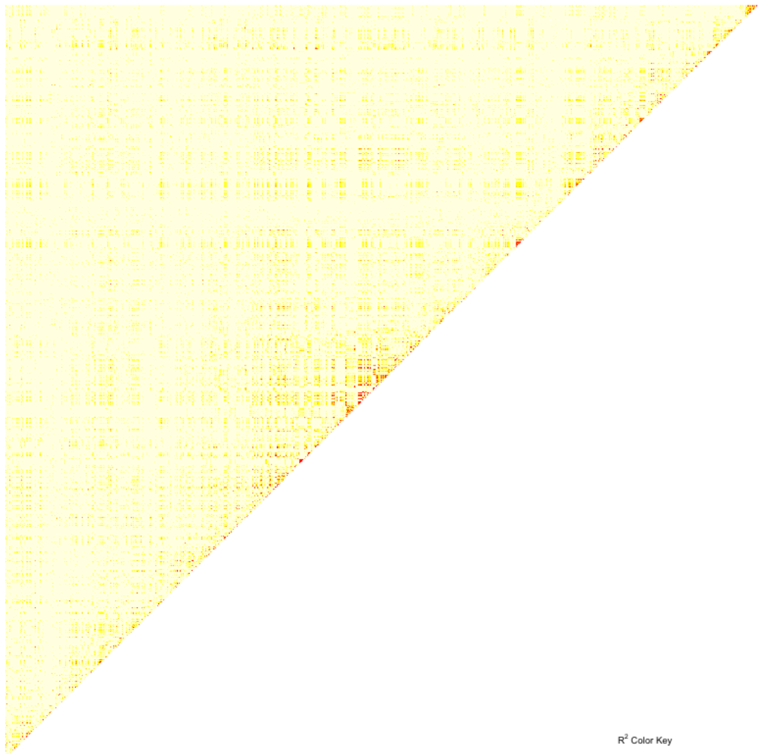
Pairwise LD in r^2 with 1301 SNPs in A06 cds range 15_to_5230 out of 5234
