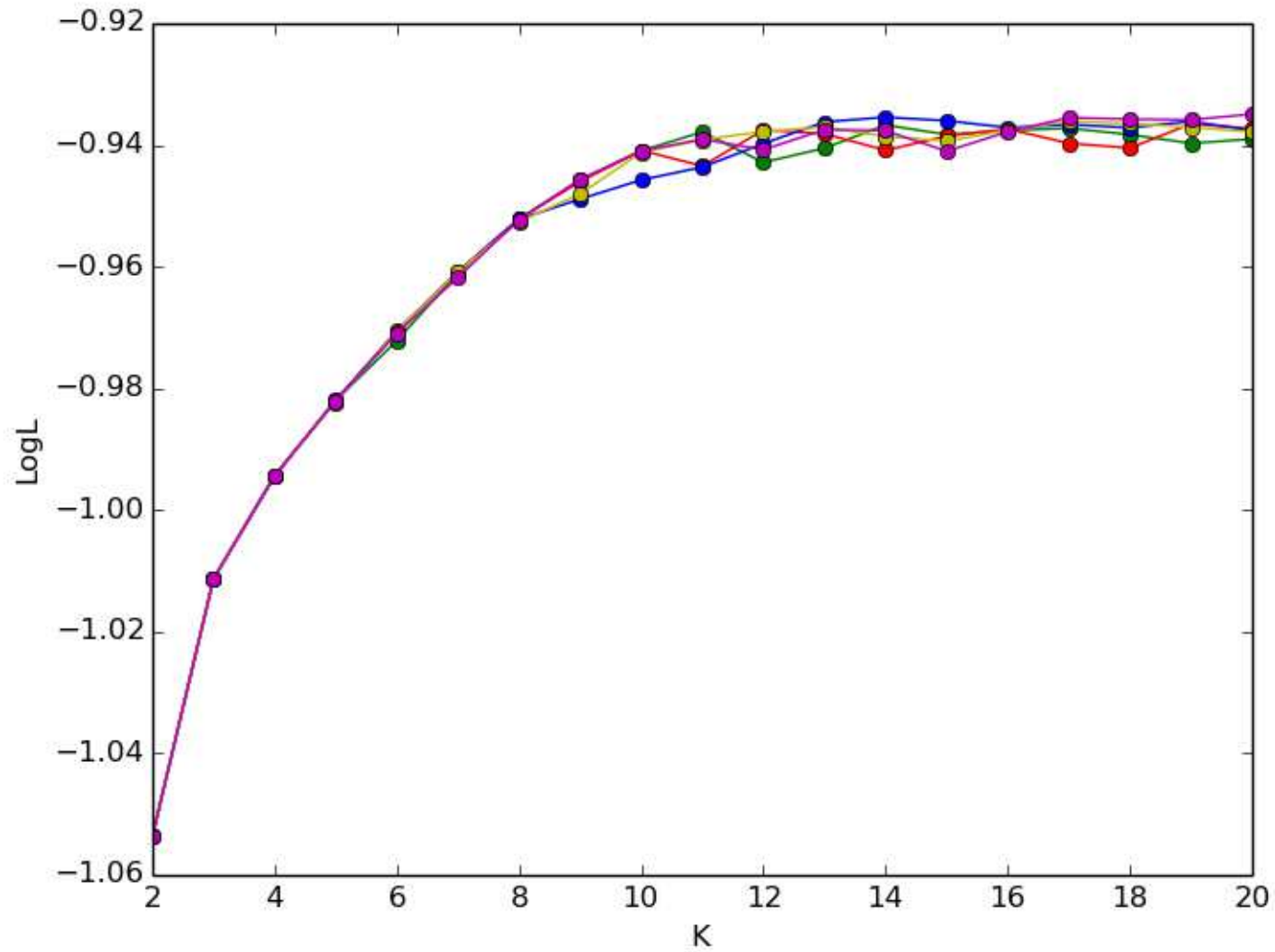
Figure S1: fastSTRUCTURE analysis. Log Likelihood of the model as a function of the number of clusters for each of the five runs
