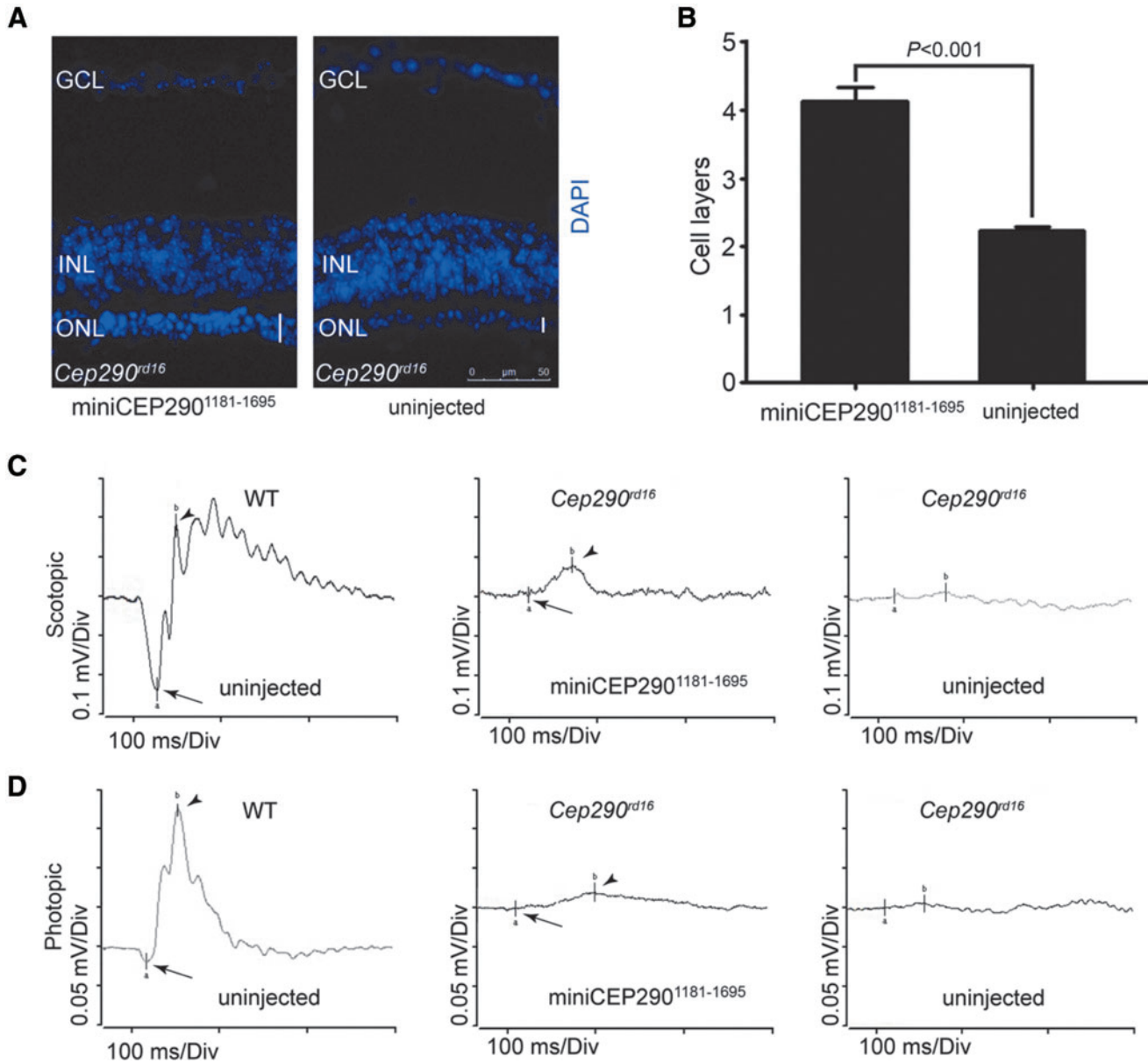
Supplementary Figure S1. In vivo rescue potential of miniCEP290 1181-1695 . (A) Cep290rd16 retinas injected with indicated miniCEP290 were stained with DAPI (blue). Age-matched uninjected Cep290rd16 retinas were used as controls. The ONL is marked with vertical lines. (B) Quantification of the ONL thickness by counting the number of layers of the virus infected region of the Cep290rd16 mice at 3 weeks post injection is represented. (C and D) Scotopic (C) and photopic (D) ERG analysis of the miniCEP290 1181-1695 injected retinas showed mild improvement at 3 weeks of age. The ERG a-wave is represented by arrows, while b-wave is depicted using arrowheads.
