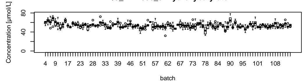
QC_EPA006_3-Hydroxybutyrate
