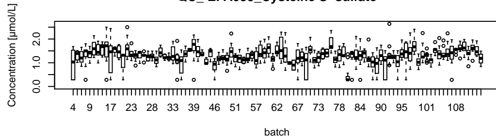
QC_EPA038_Cysteine S-sulfate
