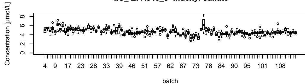
QC_EPA040_3-Indoxyl sulfate
