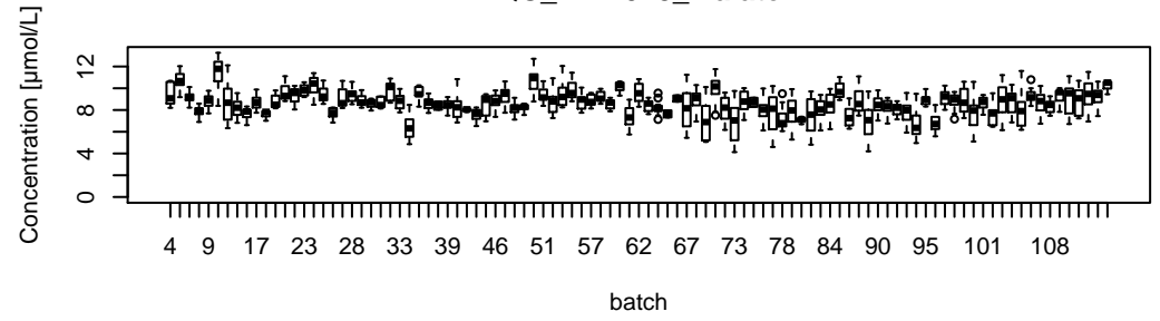
QC_EPA018_Malate
