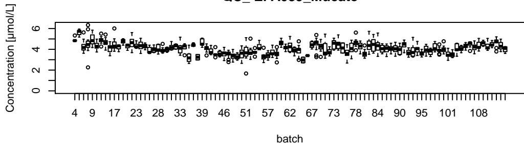
QC_EPA039_Mucate
