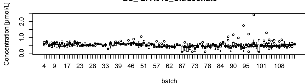
QC_EPA013_Citraconate
