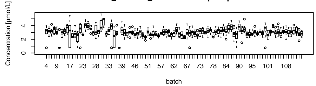
QC_EPA020_Ethanolamine phosphate
