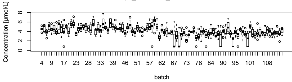
QC_EPA017_Glutarate
