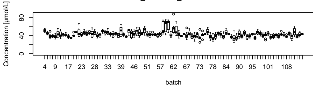
QC_EPA019_threonate
