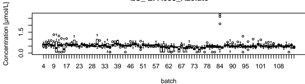
QC_EPA033_Azela
