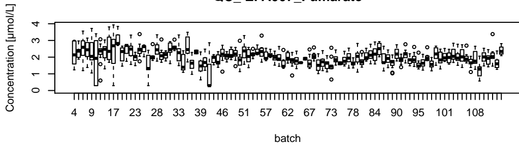
QC_EPA007_Fumarate
