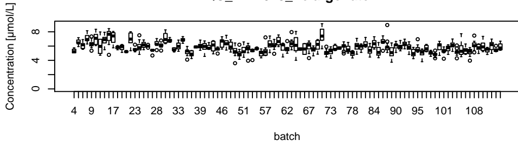
QC_EPA023_Pelargonate
