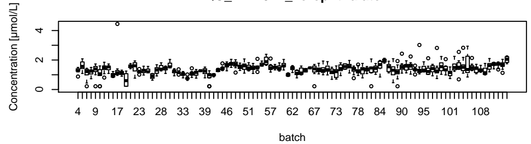
QC_EPA024_Terephthalate
