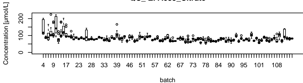
QC_EPA035_Citrate
