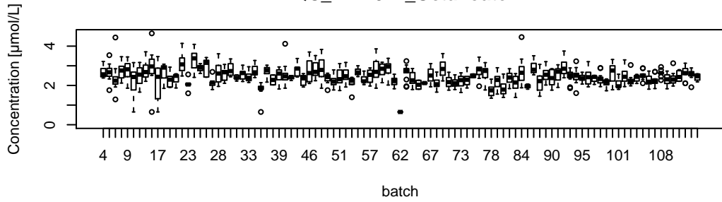
QC_EPA021_Octanoate
