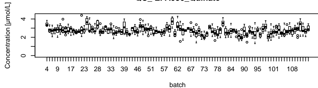
QC_EPA036_Quinate
