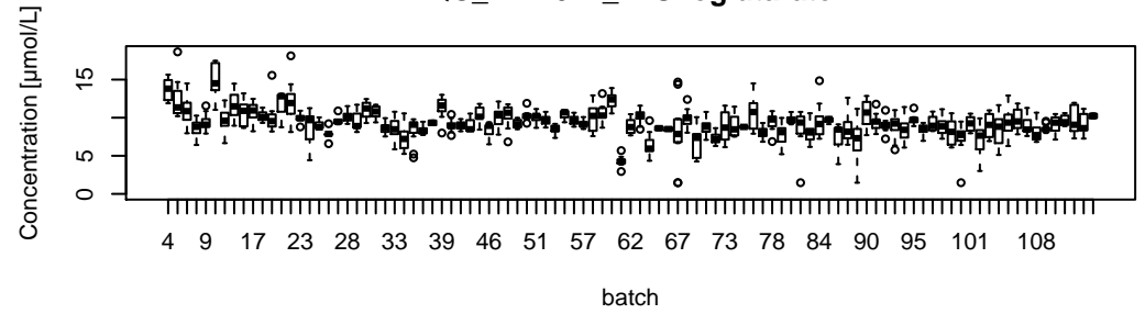
QC_EPA022_2-Oxoglutarate
