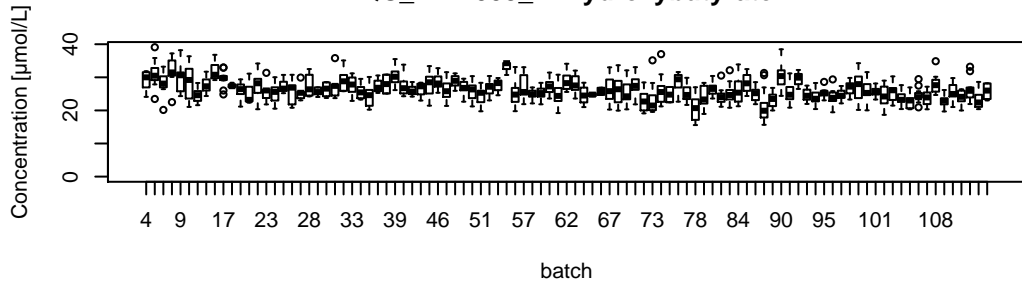
QC_EPA005_2-Hydroxybutyrate
