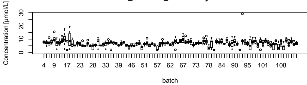
QC_EPA003_2-Oxobutyrate
