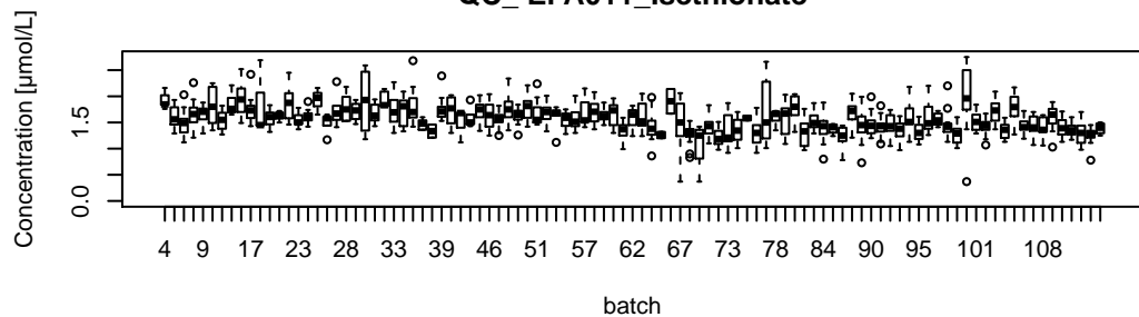
QC_EPA011_Isethionate
