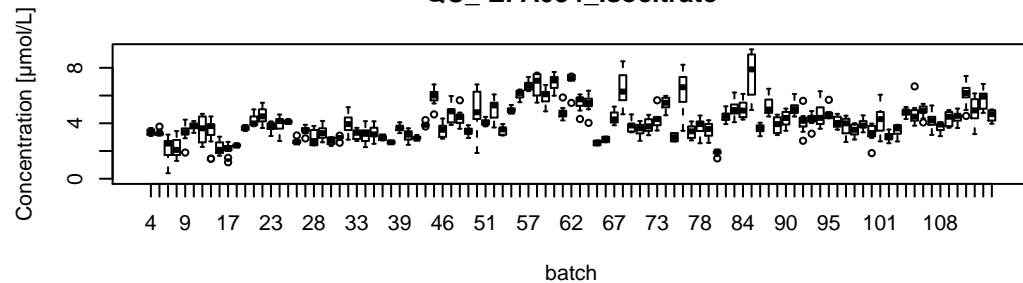
QC_EPA034_Isocitrate
