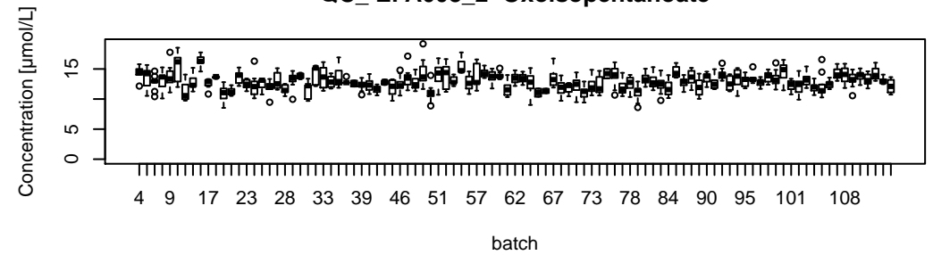
QC_EPA008_2-Oxoisopentanoate
