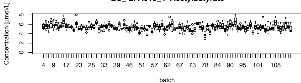
QC_EPA015_4-Acetylbutyrate
