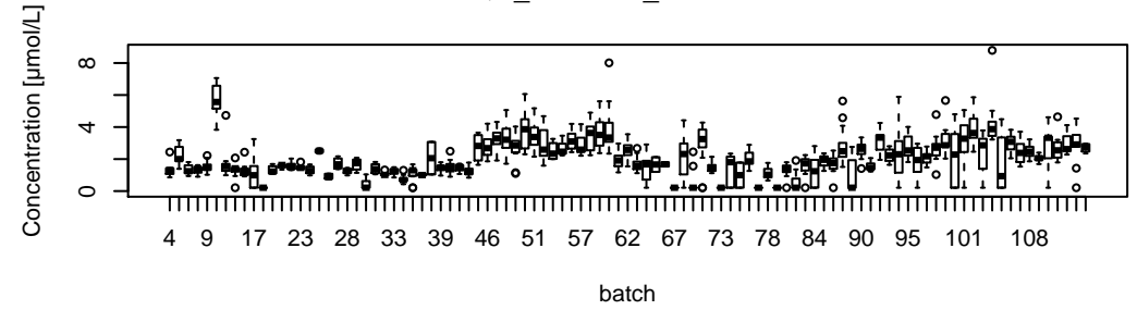
QC_EPA004_Malonate
