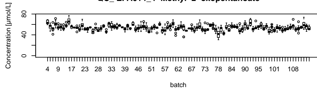
QC_EPA014_4-Methyl-2-oxopentanoate
