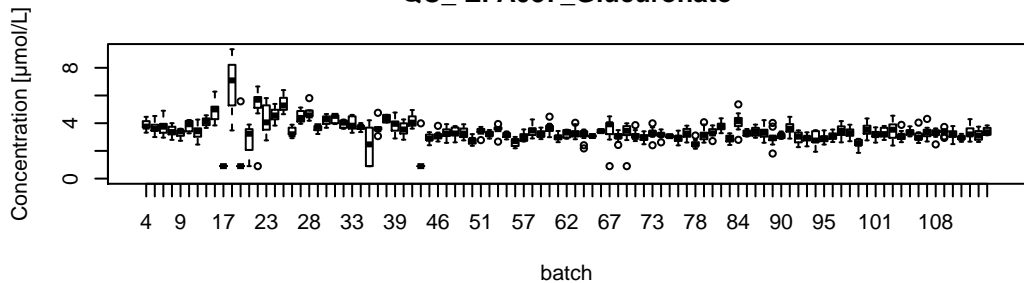
QC_EPA037_Glucuronate
