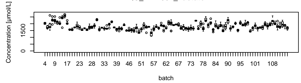
QC_EPA002_Lactate
