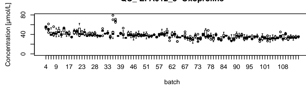
QC_EPA012_5-Oxoproline
