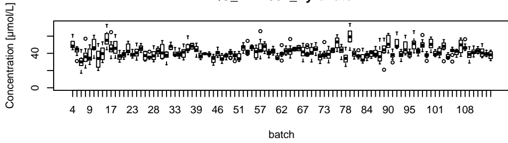
QC_EPA001_Pyruvate
