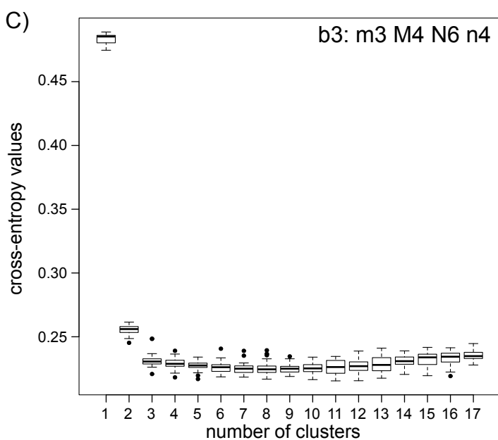
Figure S2. Standard boxplots of cross-entropy values (30 repeats) of sNMF analysis for the filtered ddRAD dataset. A, B and C show boxplots for the different stacks settings.
