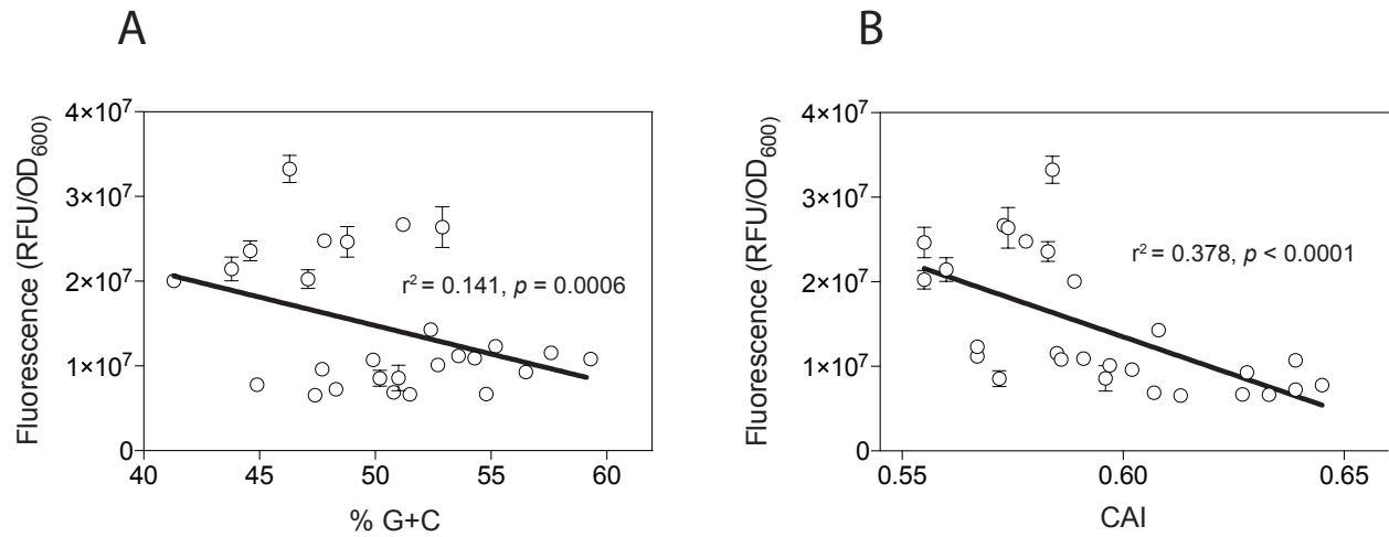
Figure S2: Association between GFP expression levels (as measured by cell fluorescence) and overall GC-content (A) or overall CAI (B) for the mosaic GFP genes. Points represent the mean \pm standard deviation of three biological replicates.
