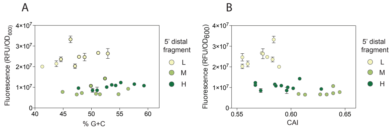
Figure S3: Association between GFP expression levels (as measured by cell fluorescence) and overall GC-content (A) or overall CAI (B) for the mosaic GFP genes. Points are colored according to the GC-content of the 5'-distal fragment as follows: yellow; 43% G+C; light green; 53% G+C; dark green; 61% G+C. Points represent the mean \pm standard deviation of three biological replicates.
