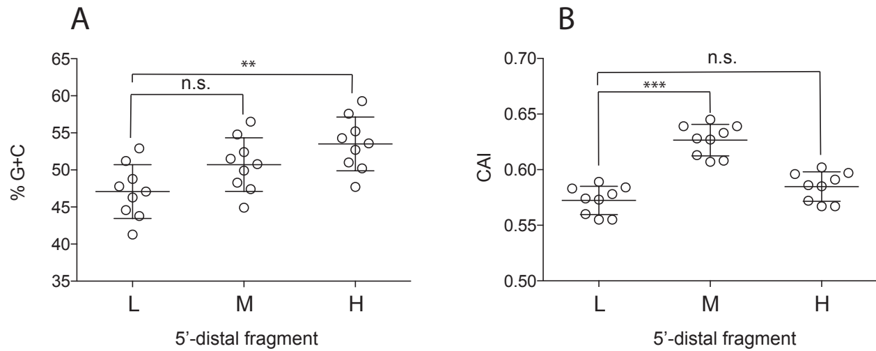
Figure S4: Comparison of overall genic GC-content ( A ) and overall genic CAI ( B ) with the GC-content of the 5'-distal fragment (L, 43% G+C; M, 53% G+C; H, 61% G+C) of the mosaic GFP genes. ** p < 0.001 , *** p < 0.0001 (Mann–Whitney–Wilcoxon test).
