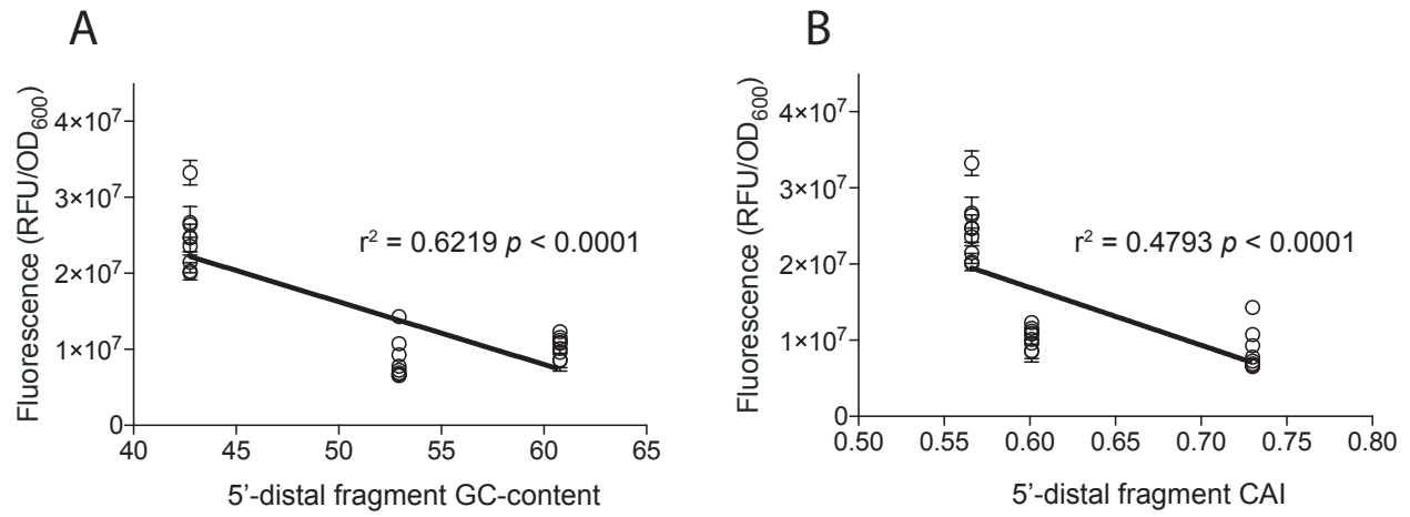
Figure S6: Association between GFP expression levels (as measured by cell fluorescence) and the GC-content (A) or CAI (B) of the 5'-distal fragment of mosaic GFP genes.
