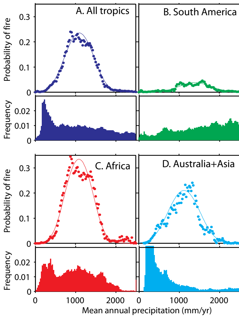
S3 Fig. The average probability that a grid cell (500x500 m) catches fire per year as a function of mean annual precipitation. The frequency distribution shows how often the precipitation class occurs. The lines are fitted logistic curves with optimum (for parameter values see Table S1). A. All tropics, B. South America, C. Africa and D. Australia and Asia.
