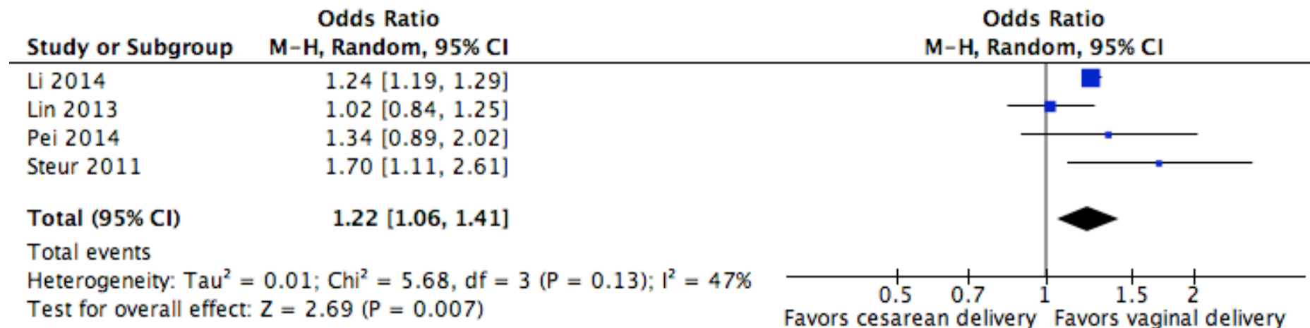
S14 Figure: A random effects meta-analysis of children being overweight at 3-8 years old after cesarean delivery compared to vaginal delivery
