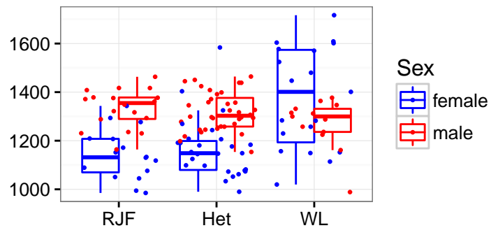
ENSGALT000000034389_LOC415708
