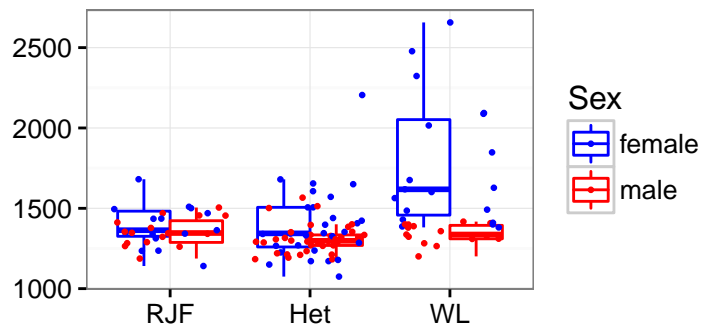
ENSGALT000000037665_RASA1
