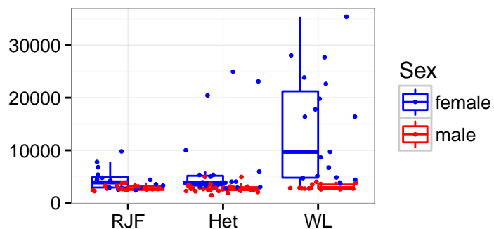
NM_204534_RARRES1
