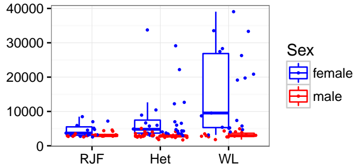
ENSGALT000000039113_OCX32_CHICK
