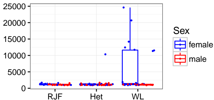
ENSGALT000000024133_COAA1_CHICK
