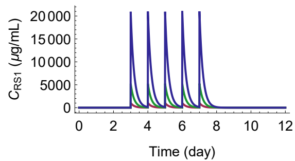
Figure S1: Simulated median exposure profiles using a one-compartment pharmacokinetic model with parameter estimates from Table S1. Doses of 10 mg/kg (red), 50 mg/kg (green), or 200 mg/kg (blue) were administered on days 3,4,5,6, and 7
