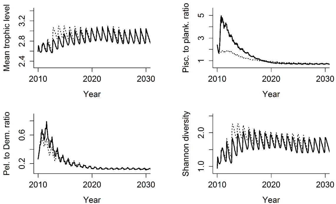
S9 Fig. Ecosystem indicators for the no-oil scenario (dotted line) and oiled scenario [K1000 \beta 363] (solid line). Mean trophic level of ecosystem, pelagic-to-demersal biomass ratio for fish, piscivorous-to-planktivorous biomass ratio for fish, and Shannon biodiversity.
