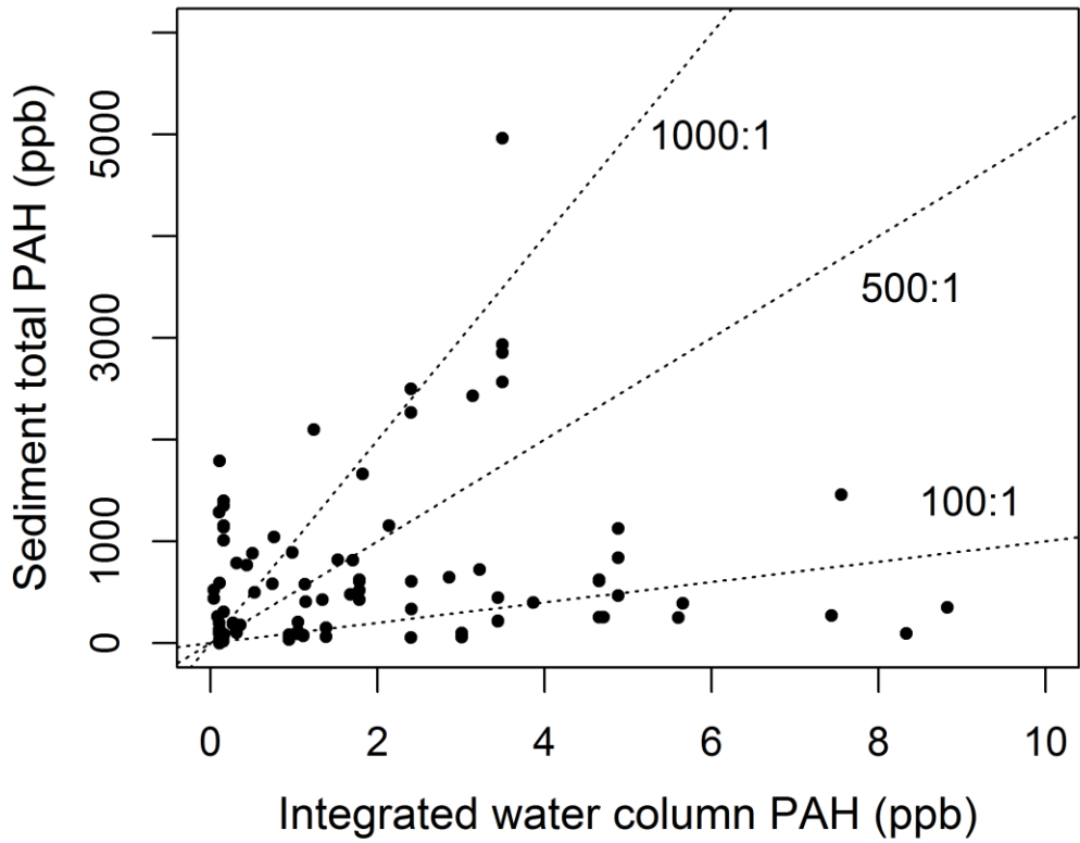
S13 Fig. Sediment PAH concentration measured in C-IMAGE sediment sampling (Romero and Hollander, unpublished data) versus time- and depth- integrated water column PAH concentrations from the Coastal Modeling System (Paris et al. 2012). Dotted lines show sediment:water column ratios for reference.
