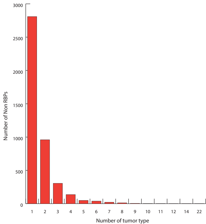
B Frequency Plot of Candidate Non-RBP drivers
