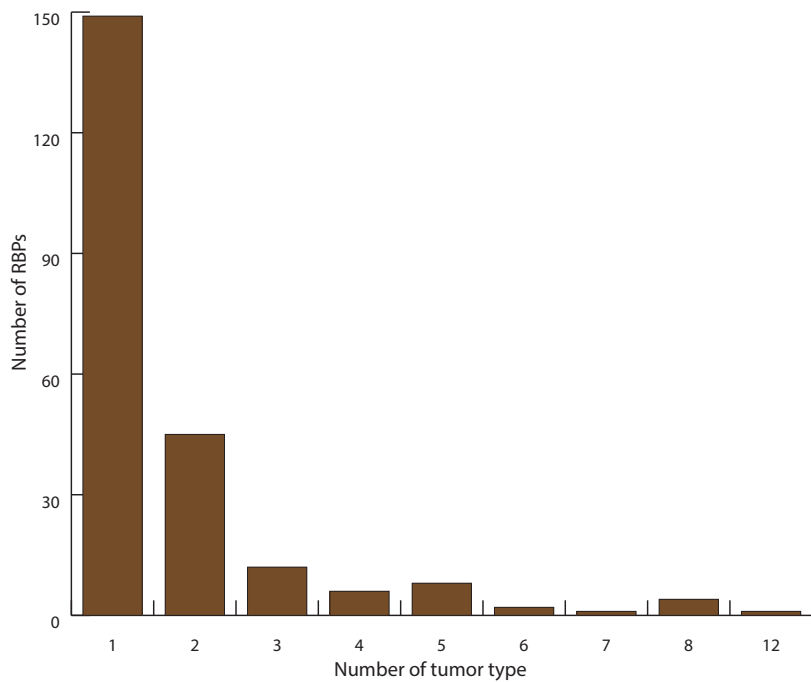
C Mutation diagram
