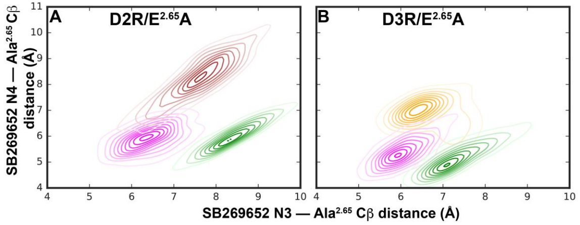
S3 Fig. Distribution of the distances from the N3 and N4 atoms of SB269652 to the C \beta atom of Ala 2.65 in mutant receptors. The MSs for each condition are colored according to Fig 1.
