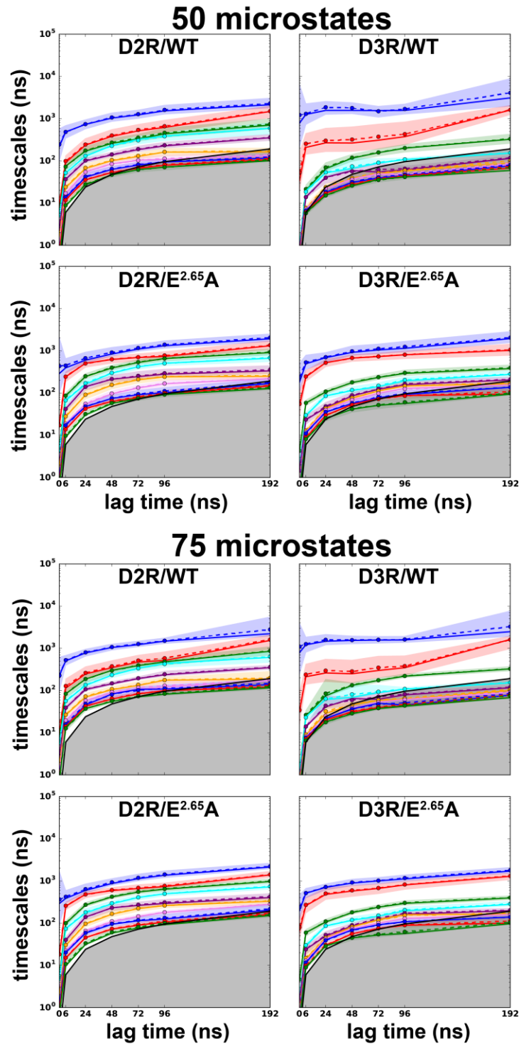
S6 Fig. Implied time scales for 50- and 75-microstate MSMs. Implied timescales (ITS) are plotted against lag time. The ITS of the maximum likelihood Bayesian Markov model are shown in solid lines, whereas the means and the 95% confidence intervals (computed by Bayesian sampling) are shown in dashed and shaded areas, respectively. In blue, red, and green, ... are the 1 st , 2 nd , and 3 rd , ... slowest ITS.
