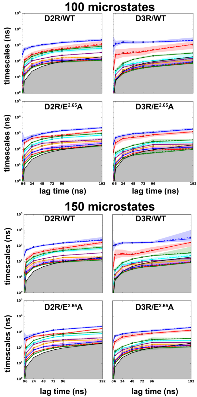
S7 Fig. ITS for 100- and 150-microstate MSMs. The color coding is the same as in S6 Fig.
