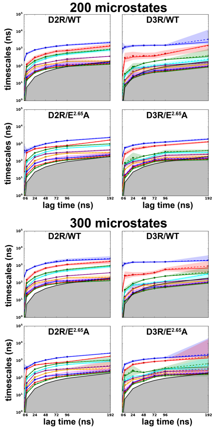
S8 Fig. ITS for 200- and 300-microstate MSMs. The color coding is the same as in S6 Fig.
