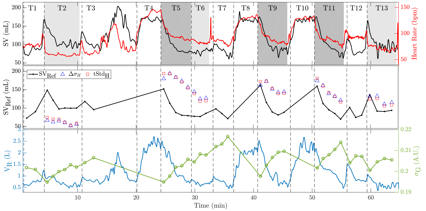
Fig S5. Temporal evolution of SV_{Ref} , heart rate and EIT-based features for subject S06. See caption of Fig. 9 for details.
