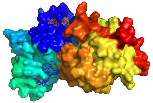
(b) Apo-LieIF trunc /MD
