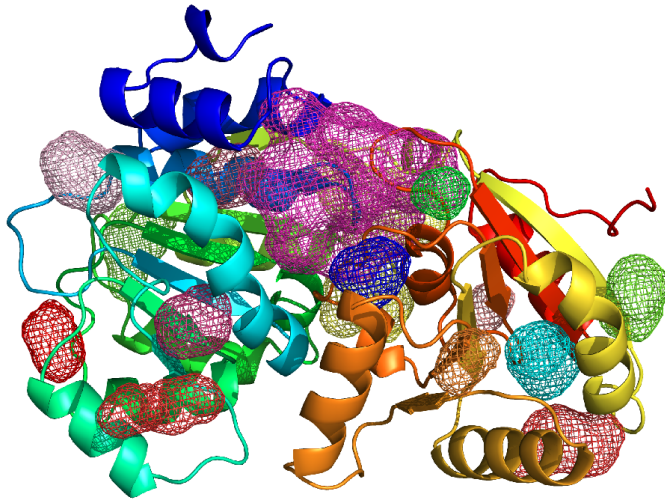
(c) Holo-LieIF trunc /MD
