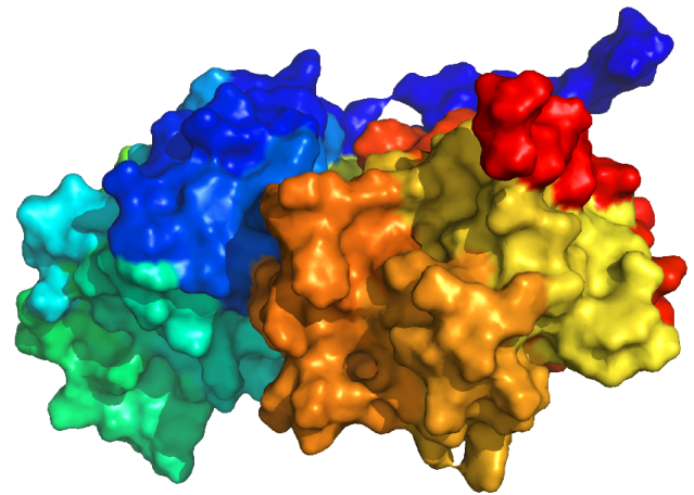
(f) Human eIF4AI
