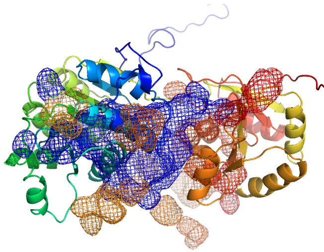
(a) Apo-LieIF trunc /MD
