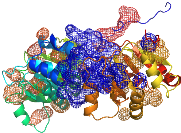
(e) Human eIF4AI
