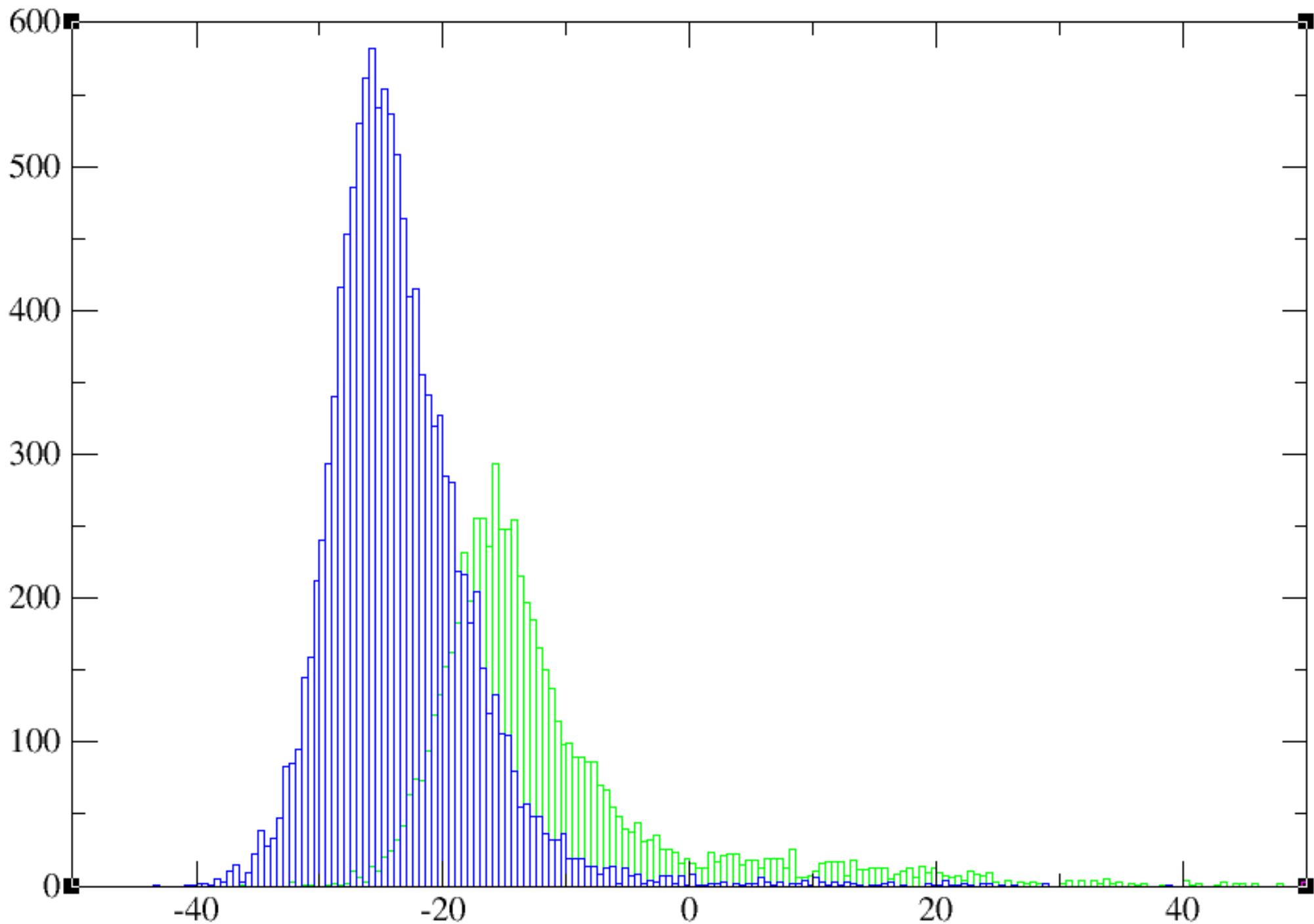
Dock scores on pocket P2
